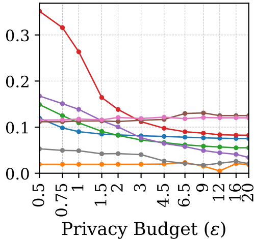
Closeness Centrality Distribution Error
